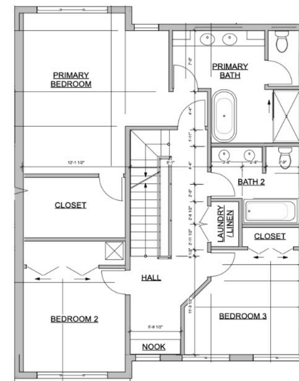
1 BUILDING 1, LEVEL 2 INTERIOR DIMENSIONS (UNIT 1A MIRRORED)
