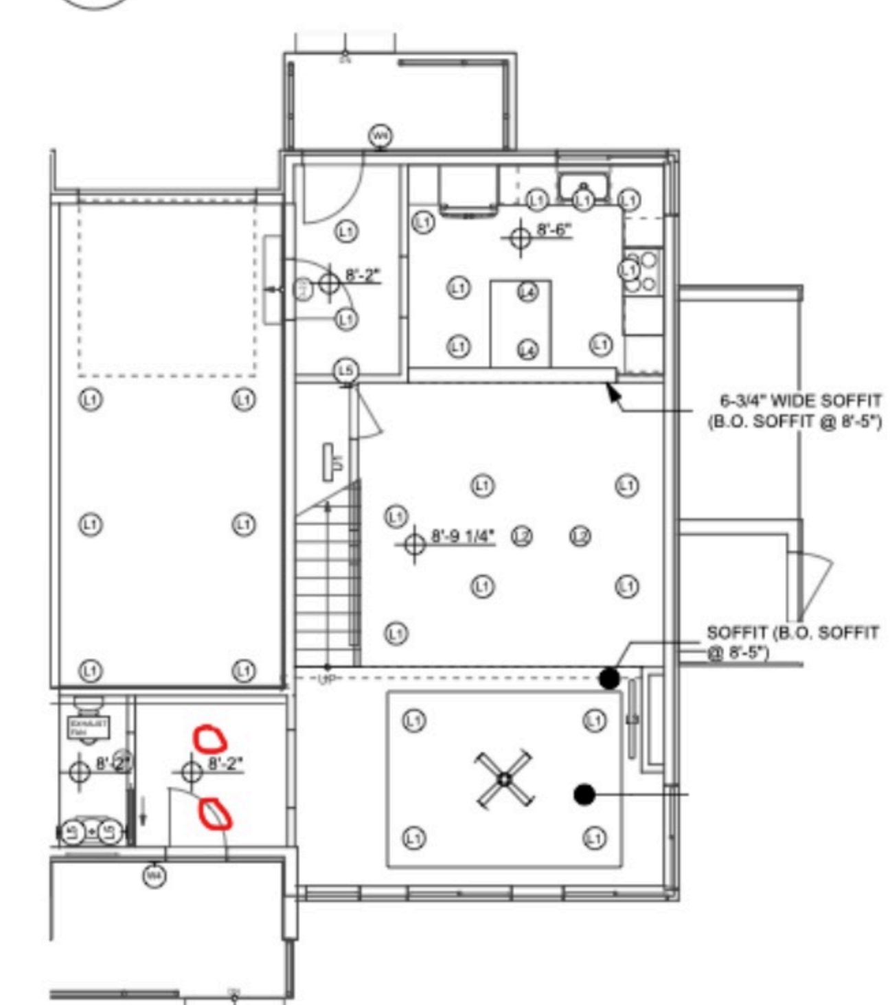
1 LEVEL 1 RCP, TYPICAL
