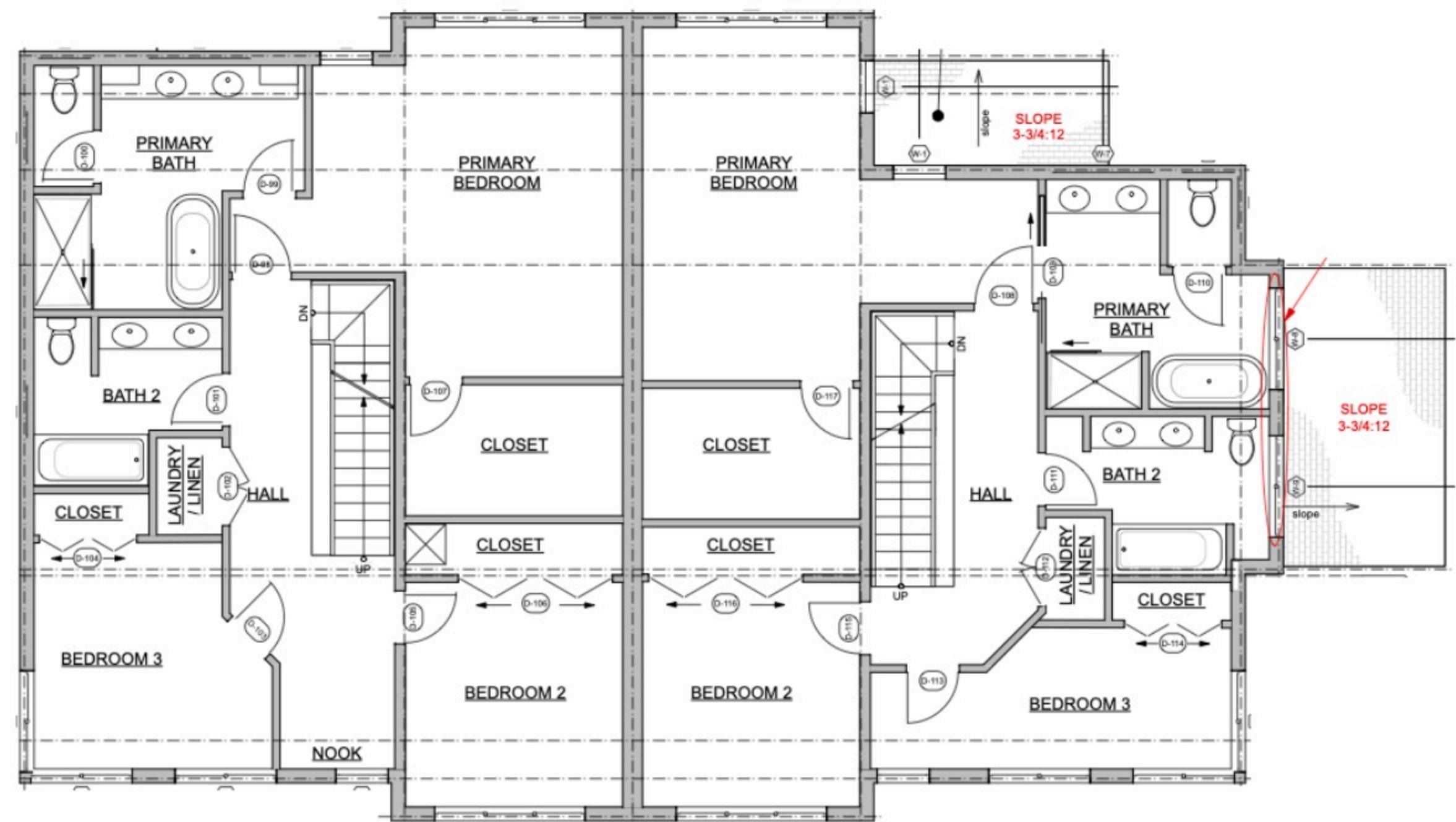
1 LEVEL 2 PLAN BUILDING 2 & 3
