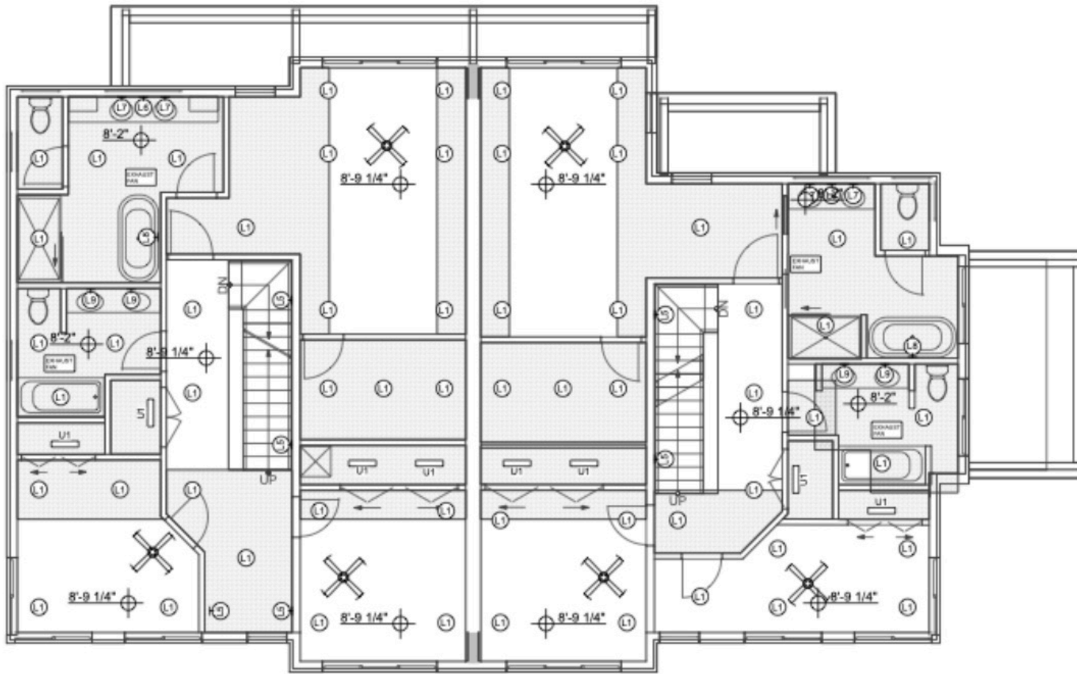
5 LEVEL 2 RCP
