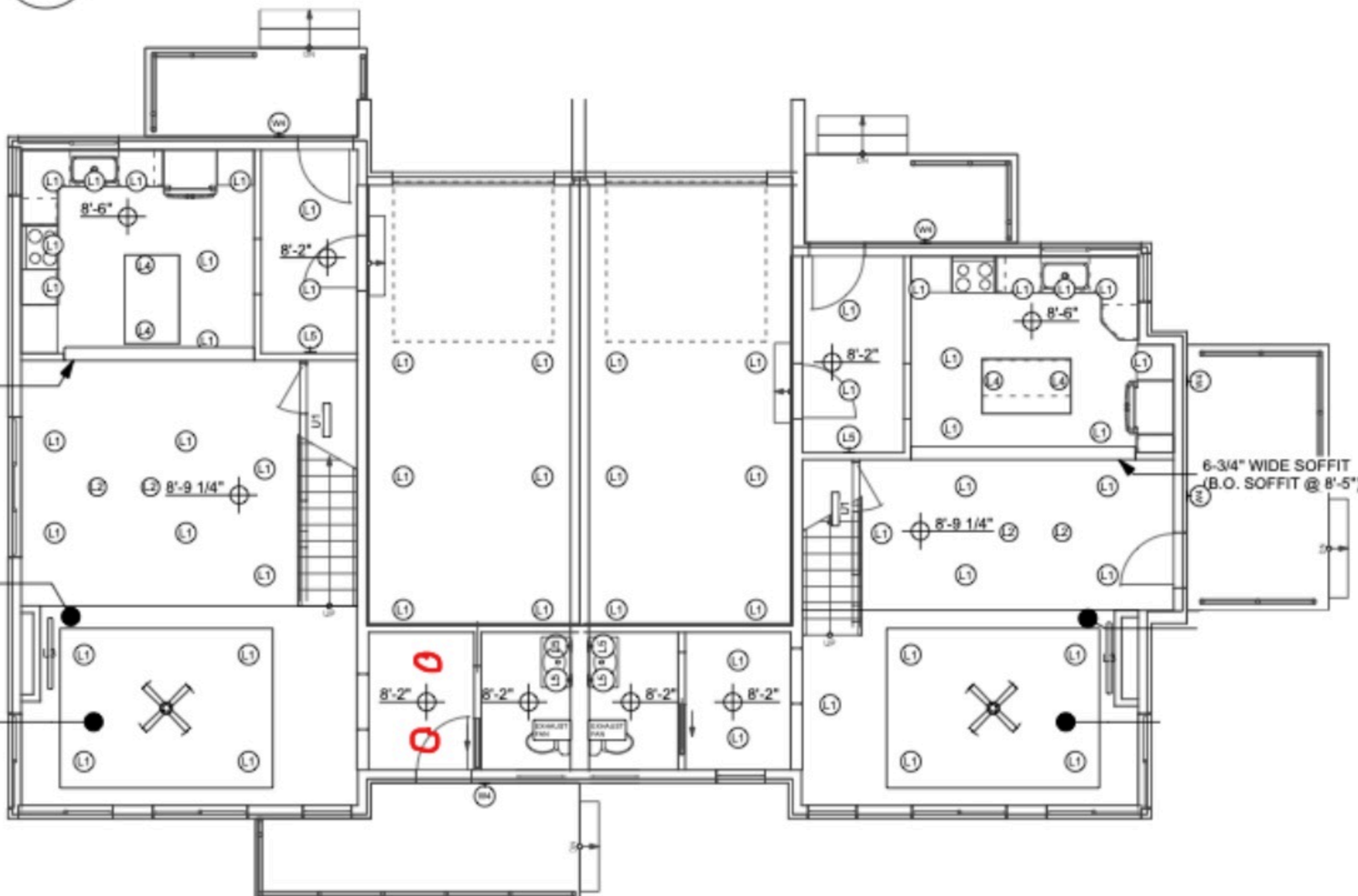
4 LEVEL 1 RCP
