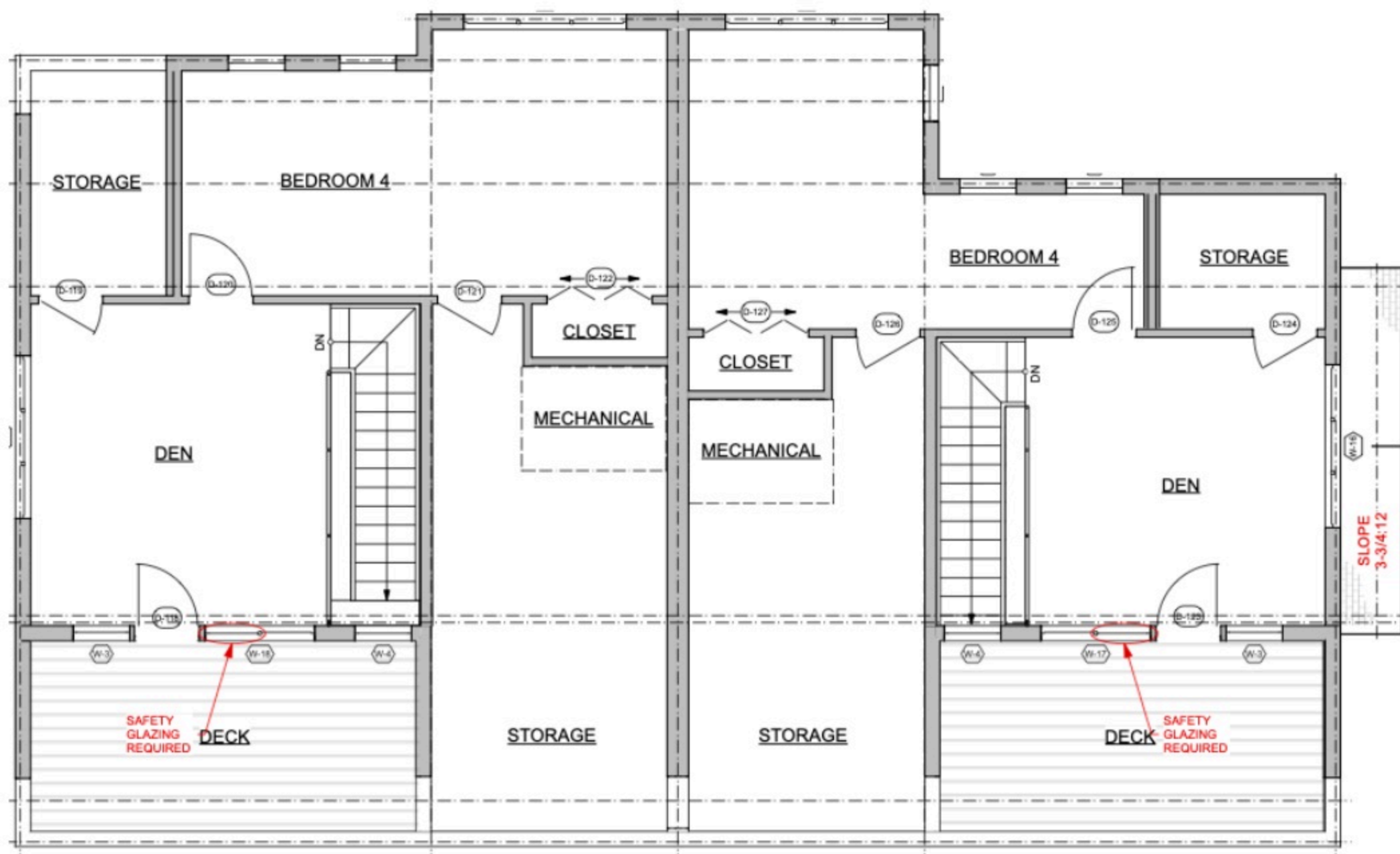
2 LEVEL 3 PLAN BUILDING 2 & 3
