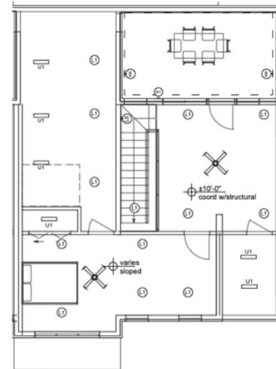
3 LEVEL 3 RCP, TYPICAL
