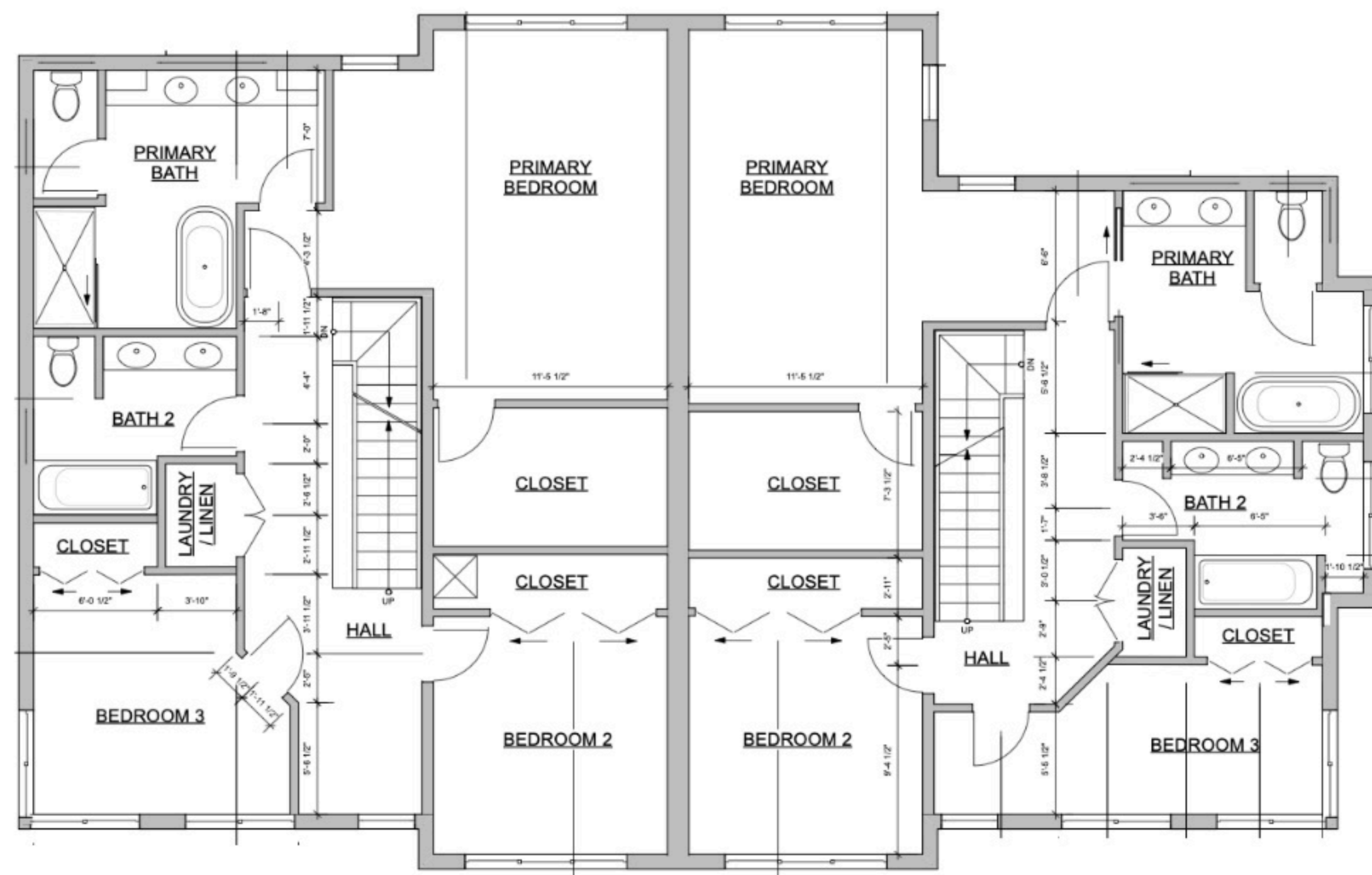
2 BUILDINGS 2 & 3 LEVEL 2 INTERIOR DIMENSIONS, TYPICAL
