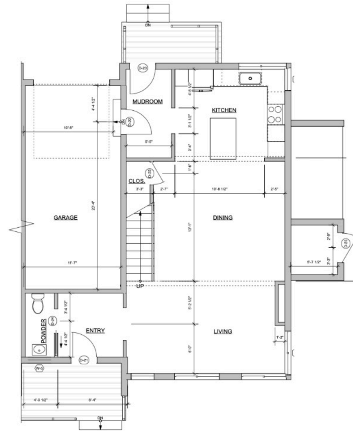
1 BUILDING 1, LEVEL 1 INTERIOR DIMENSIONS (UNIT 1A MIRRORED)
