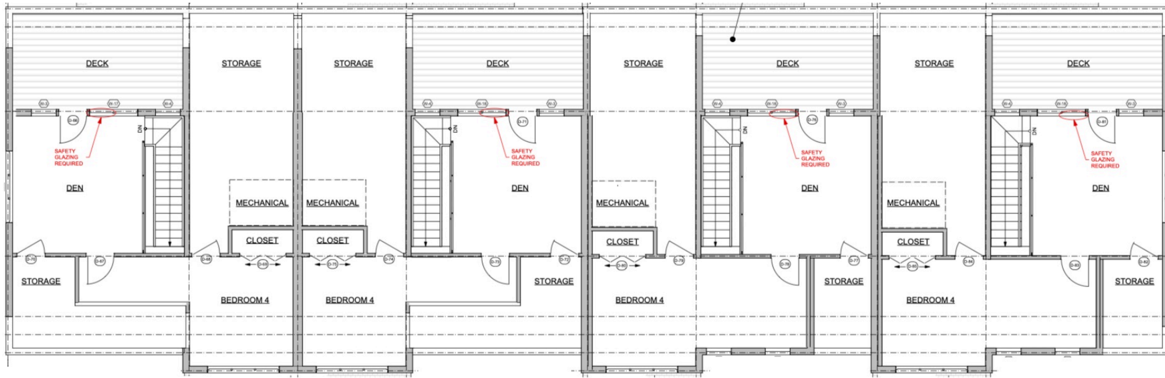
1 LEVEL 3 PLAN - BUILDING 1
