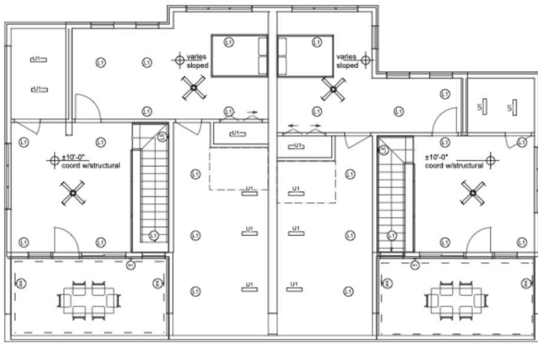
6 LEVEL 3 RCP
