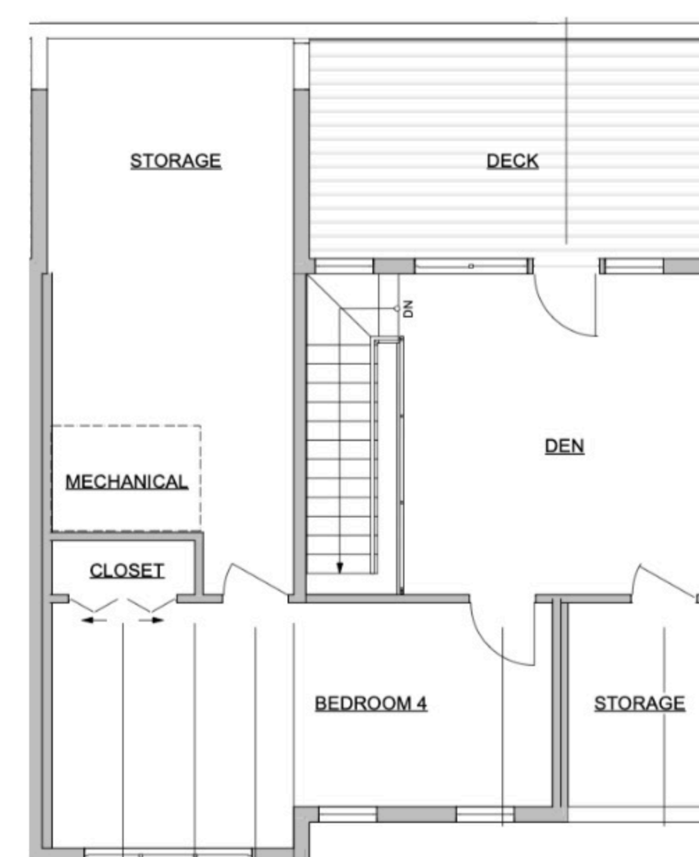
1 BUILDING 1, LEVEL 3 INTERIOR DIMENSIONS (UNIT 1A MIRRORED)
