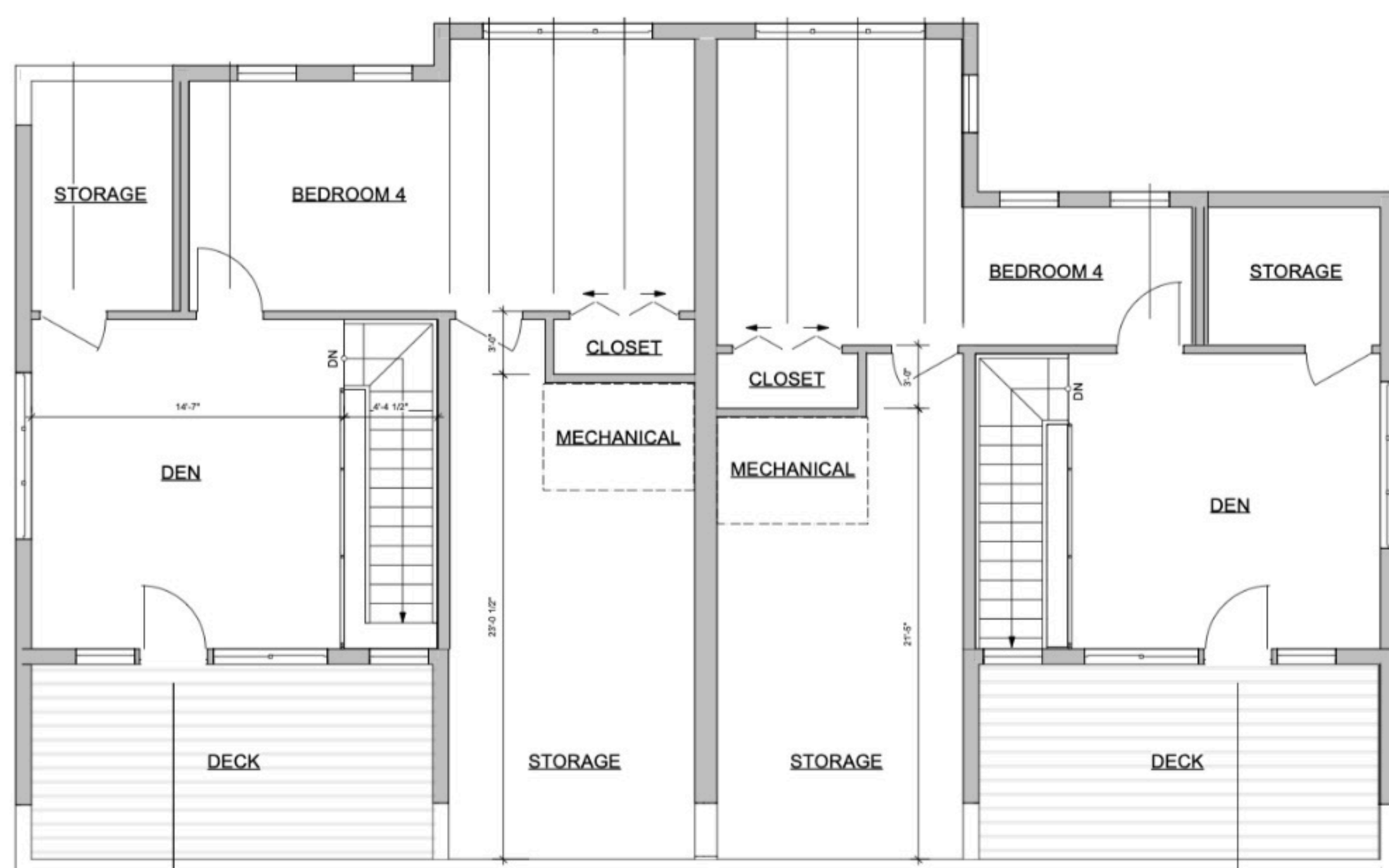
2 BUILDINGS 2 & 3 LEVEL 3 INTERIOR DIMENSIONS, TYPICAL
