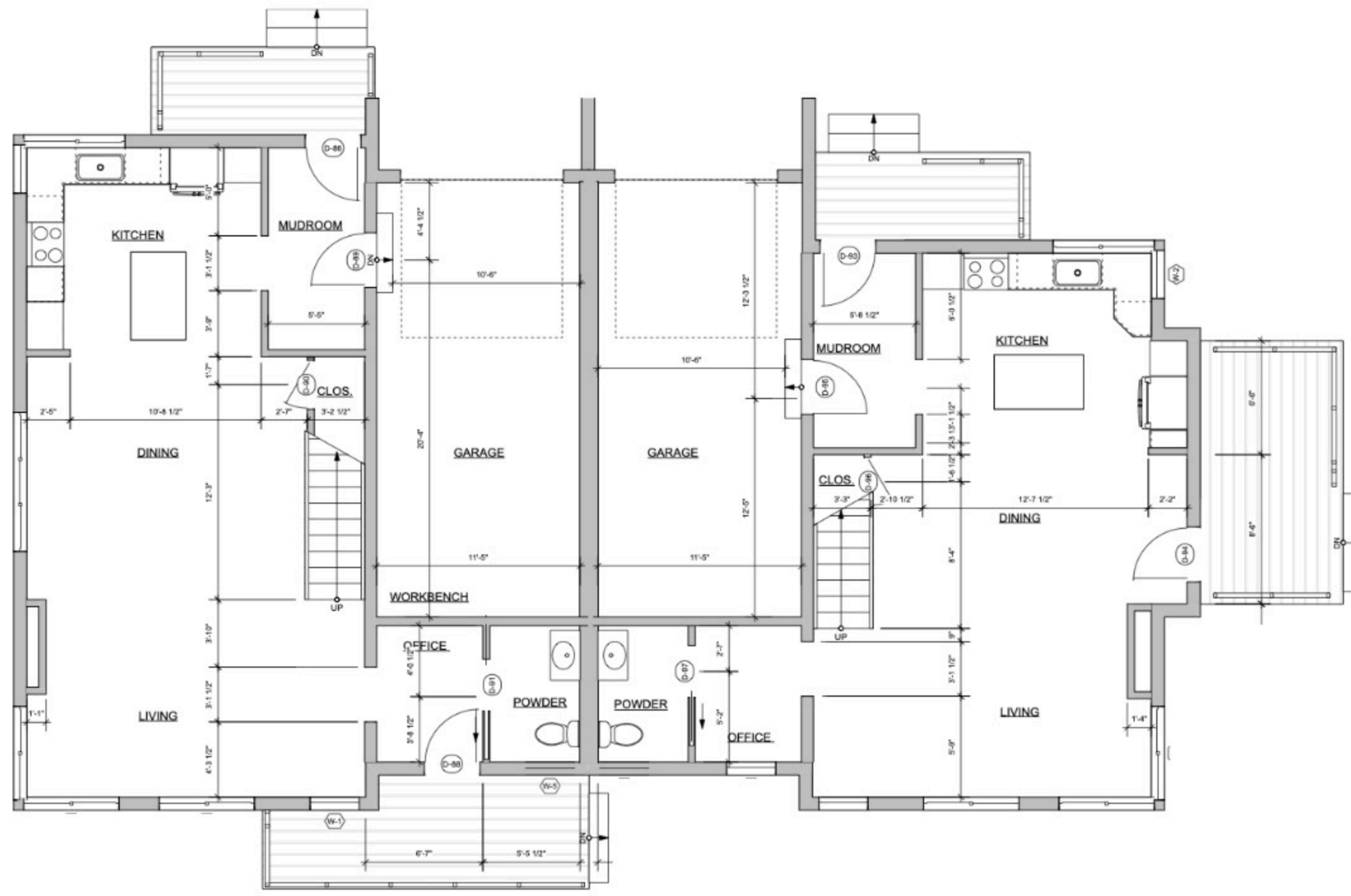
2 BUILDINGS 2 & 3 LEVEL 1 INTERIOR DIMENSIONS, TYPICAL
