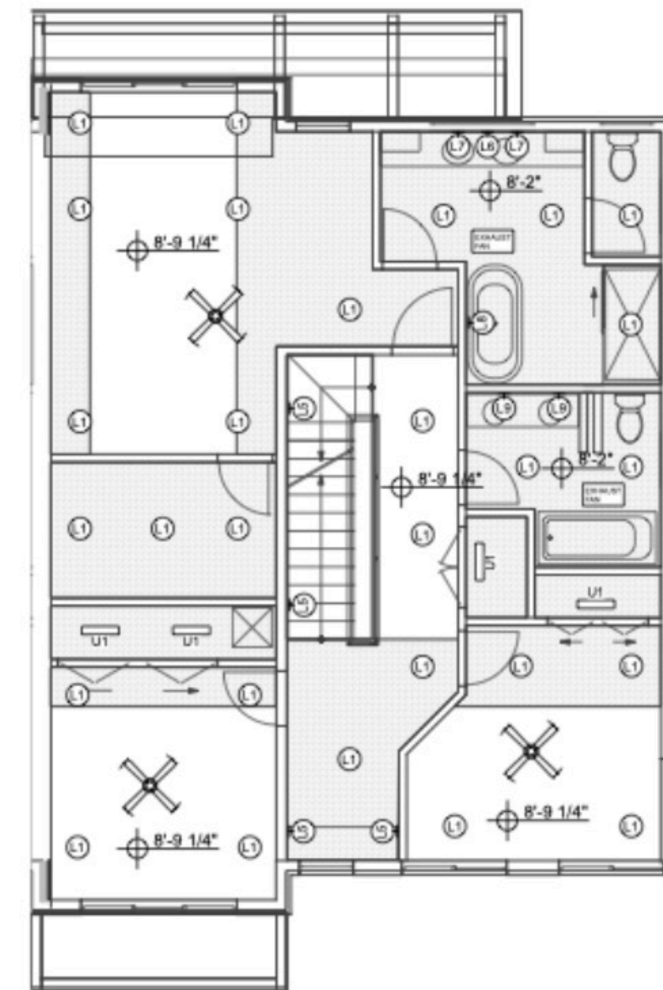
2 LEVEL 2 RCP, TYPICAL
