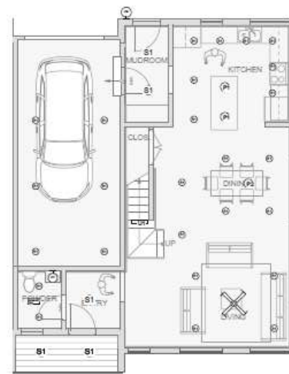
1 LEVEL 1 RCP, TYPICAL Scale: 1/8" = 1'-0"
